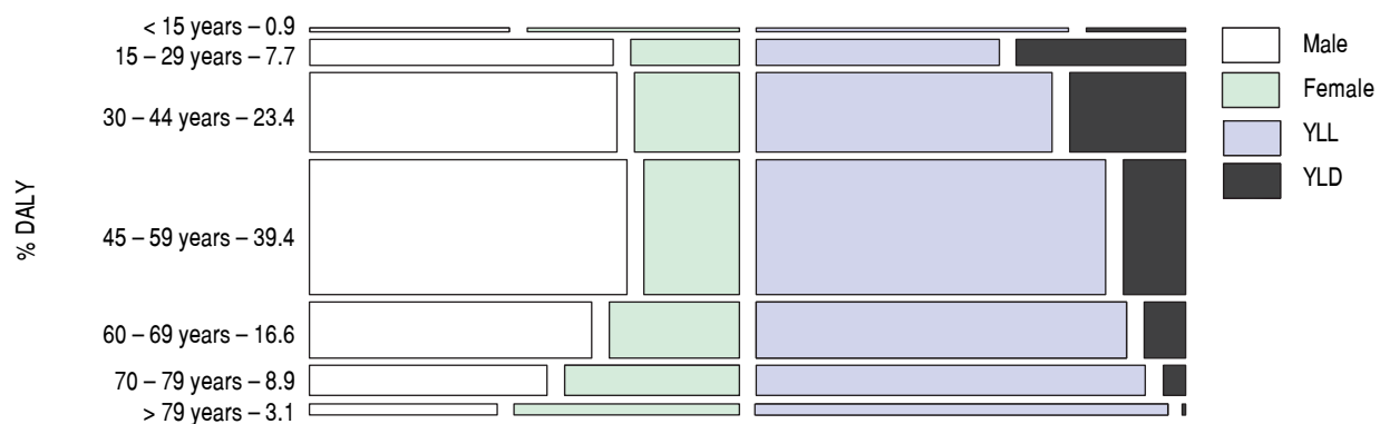
Figure 1. Chronic hepatitis B and cirrhosis due to hepatitis B – Brazil, 2008: Disability Adjusted Life Years (DALY) distribution according to gender, the proportion of Years of Life Lost (YLL) and Years Lived with Disability (YLD) and age groups (bars width indicate the proportion of each age group).
