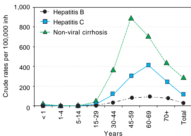
Figure 4. Years of Life Lost (YLL), Years Lived with Disability (YLD) and Disability Adjusted Life Years (DALY) according to age groups for Hepatitis B, * Hepatitis C † and non-viral cirrhosis ‡ . Brazil, 2008. * Includes chronic hepatitis B and cirrhosis due to hepatitis B. † Includes hepatitis C and cirrhosis due to hepatitis C. ‡ Includes cirrhosis from alcohol and other non-viral causes of cirrhosis.
