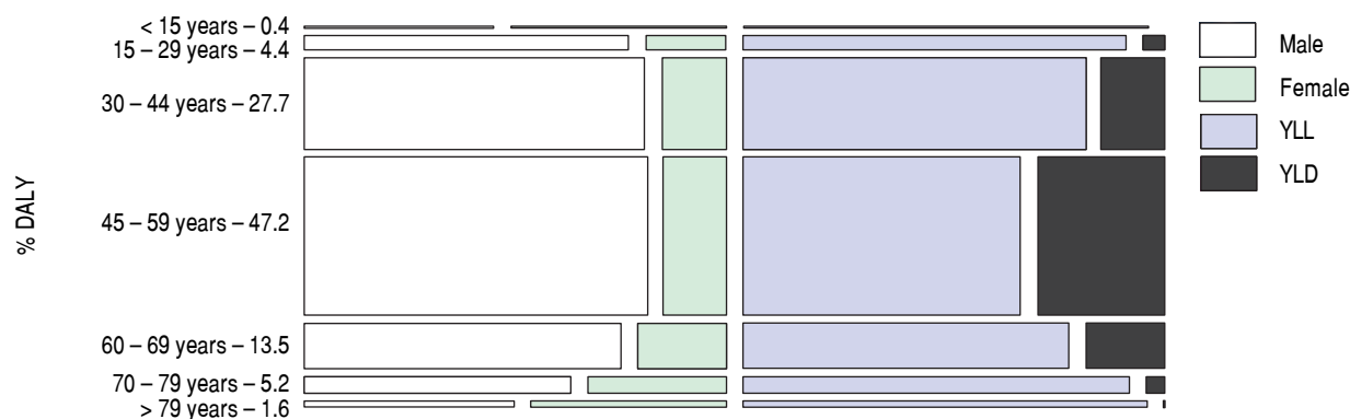
Figure 3. Non-viral cirrhosis– Brazil, 2008: Disability Adjusted Life Years (DALY) distribution according to gender, the proportion of Years of Life Lost (YLL) and Years Lived with Disability (YLD) and age groups (bars width indicate the proportion of each age group).
