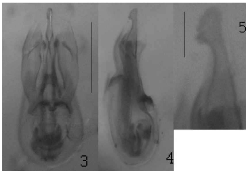
Figs. 3-5. Omalium subsolanum Herman, 2001. 3-5 – aedeagus (3 - ventral view; 4 – lateral view; 5 – apex of aedeagus laterally). Scale bar 0.1 mm (Figs. 3-4), 0.05 mm (Fig. 5).
