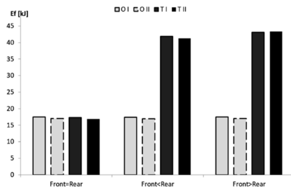
Fig. 7. Summary work of tyre friction forces during the operation of various differentials and ratios of dynamic radii of drive wheels at the distance of 1 km
