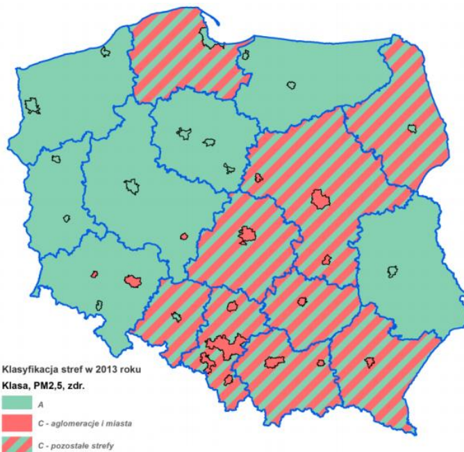
Fig. 6. Classification of zones in Poland for PM2.5 for 2013 (the protection of human health)
