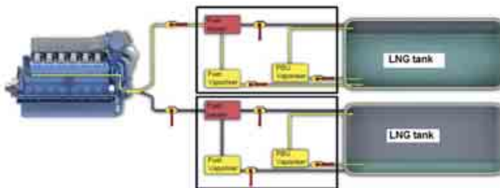
Fig. 2. The LNG fuel supplying installation (tank room arrangement) [1]
