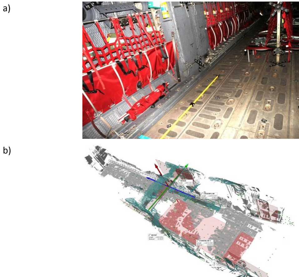
Fig.3. The cargo area of the C-130 transport aircraft, a) the real view, b) the scanned view of the aircraft interior
